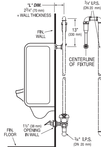
Model 323 — Water Saver (1.5 gpf/5.7 Lpf) Model 323-1.0 Low Consumption (1.0 gpf/3.8 Lpf)
