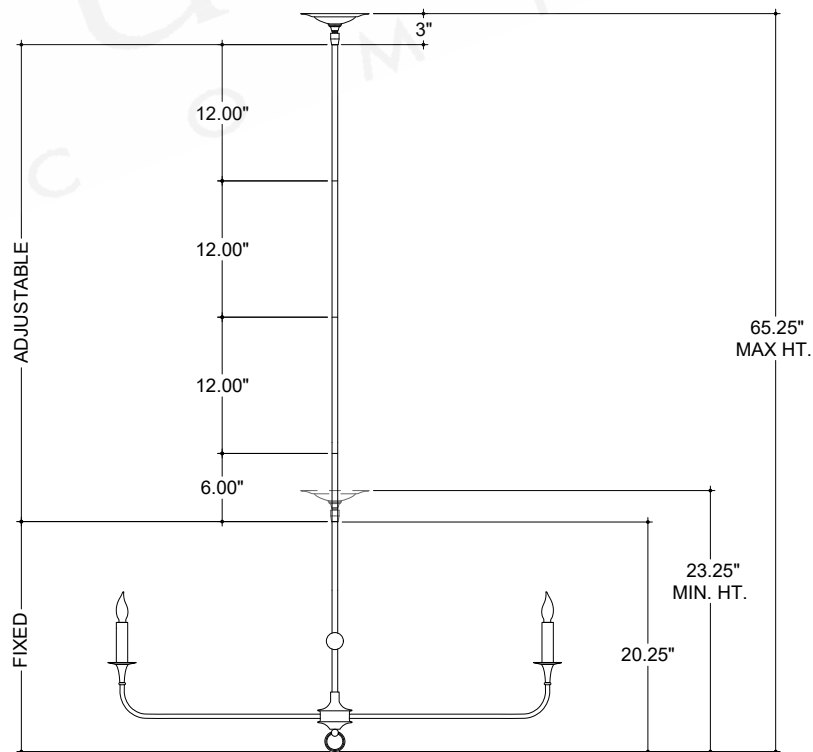
FRONT VIEW
