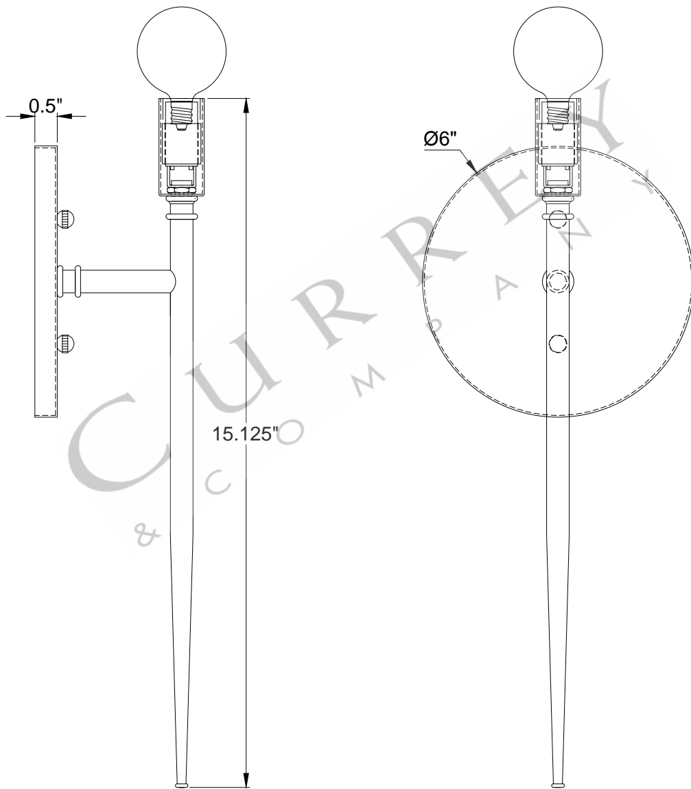
SIDE VIEW
