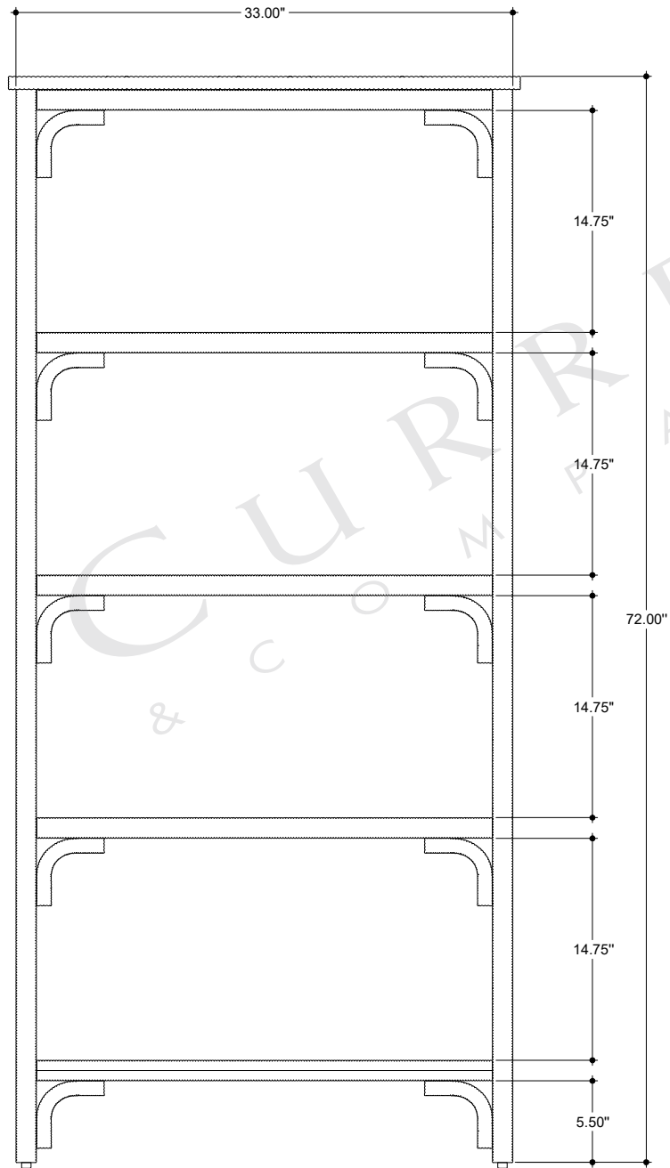
FRONT VIEW
