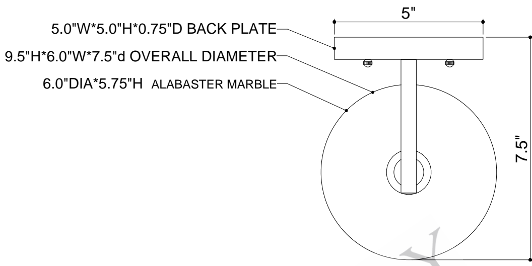
TOP VIEW
