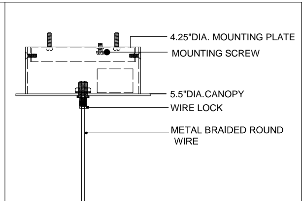
CANOPY DETAIL
