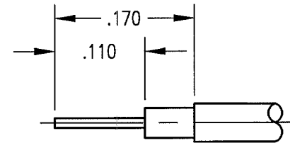
CABLE TRIMMING DIMENSIONS
