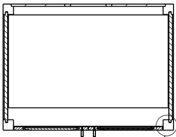
SECTION D-D SEE DETAIL C
