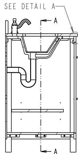
SECTION B-B SEE DETAIL A
