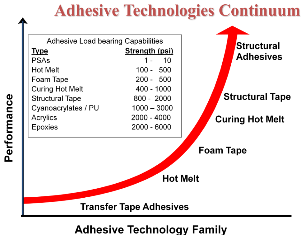
Figure 1: Adhesive technology families. Different types of adhesives vary significantly in their load-bearing capability (strength); ranging from familiar technologies such as pressure sensitive adhesives frequently applied to tapes, up through various liquid adhesive technologies (hot melts for example); with epoxy adhesives generally being the strongest category of adhesive. This chart deals only with load-
