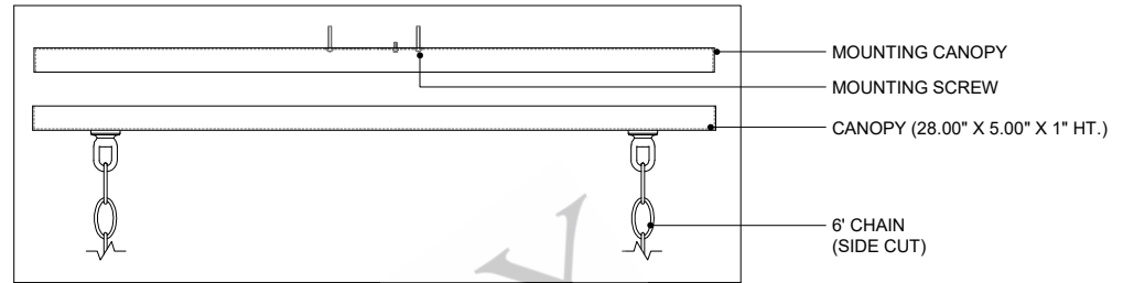
CANOPY DETAIL
