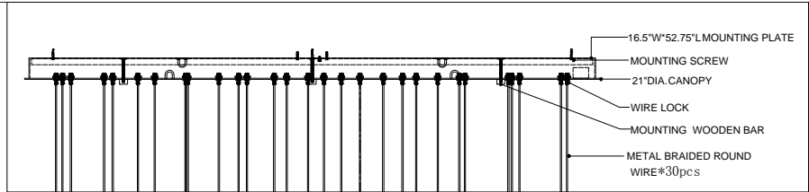
CANOPY DETAIL
