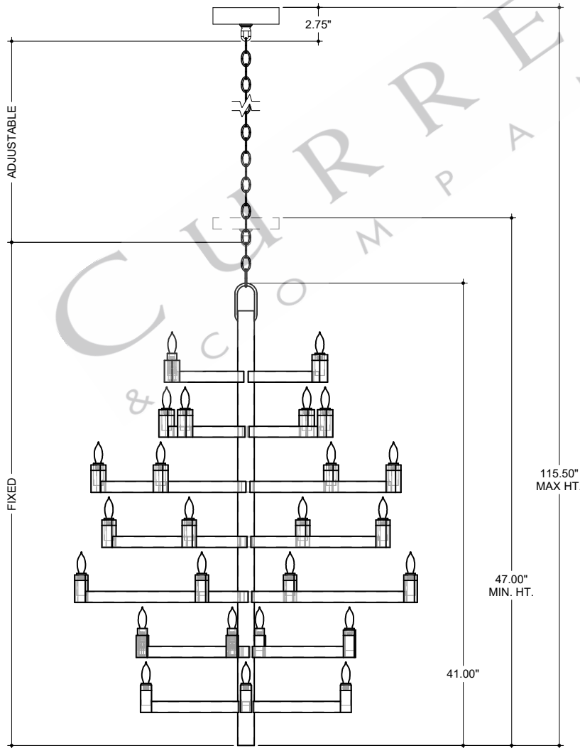
FRONT VIEW
