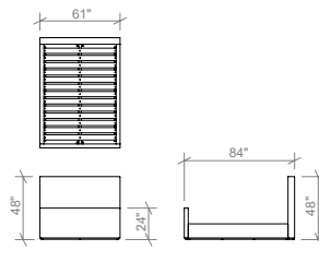
FULL BED WITH FOOTBOARD EL-E006-FF
