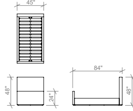
TWIN BED WITH FOOTBOARD EL-E006-TF
