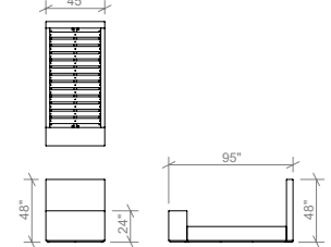
TWIN BED WITH BENCH EL-E006-TB
