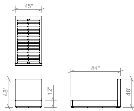
TWIN BED EL-E006-T
