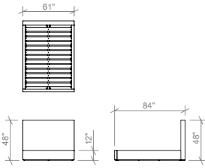
FULL BED EL-E006-F
