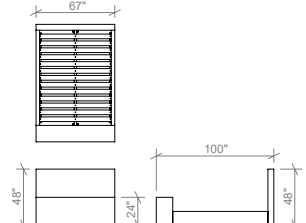
QUEEN BED WITH BENCH EL-E006-QB
