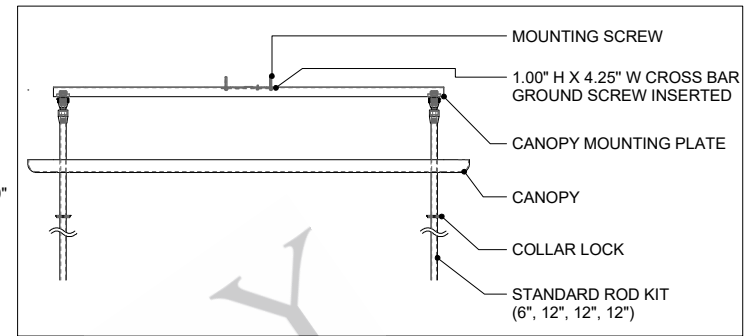
CANOPY DETAIL
