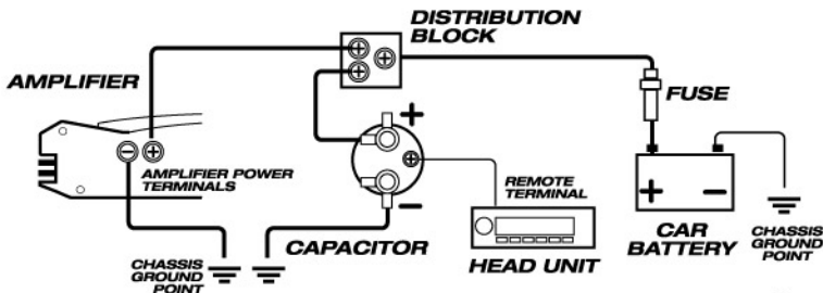
SUGGESTED WIRING
