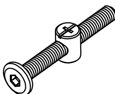
ALLEN KEY BOLT & CROSS NUT M6 X 45mm QTY 4 SETS
