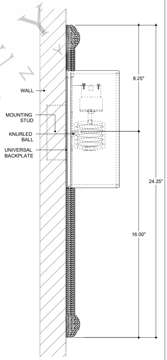
SIDE VIEW
