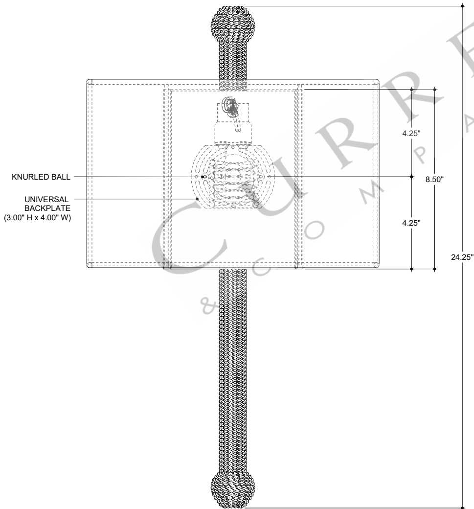
FRONT VIEW
