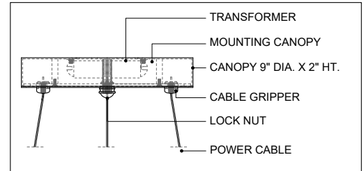
CANOPY DETAIL
