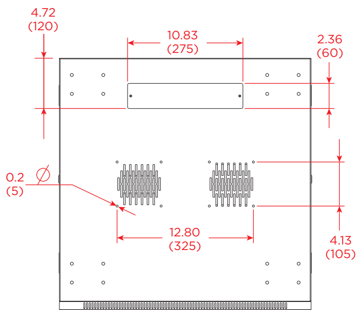
TOP/BOTTOM VIEW
