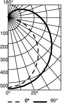
FMVCCLS 36IN , input watts 26.39, test no. ISF 37684
