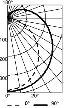
FMVCCLS 24IN , input watts 18.12, test no. ISF 37684
