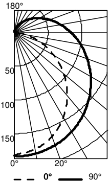
FMVCCLS 12IN , input watts 9.61 test no. ISF 37684
