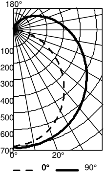
FMVCCLS 48IN , input watts 34.86, test no. ISF 37684
