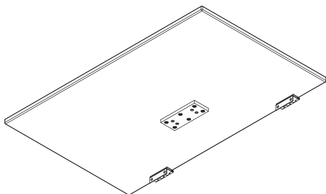
E. Top Panel x 1 Panel superior x 1 25923
