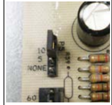
FIGURE 32 - JUMPER P5
