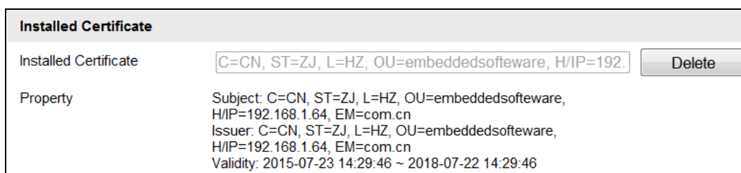
Figure 5-24 Installed Certificate
