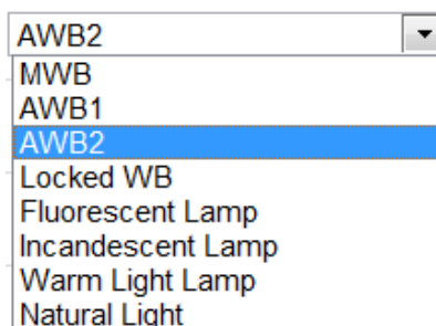
Figure 5-30 White Balance
