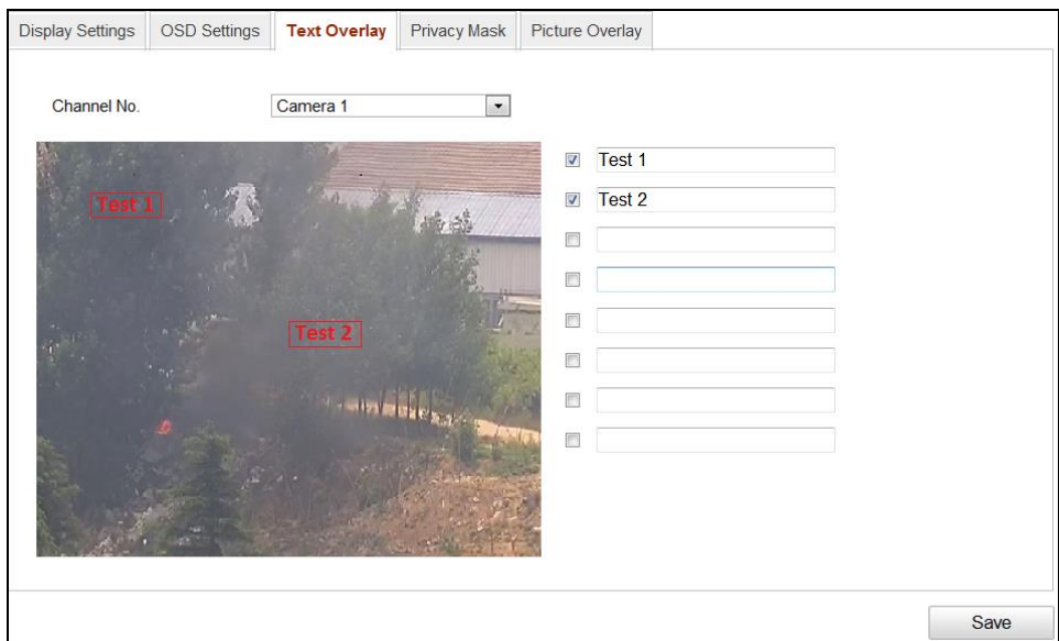
Figure 5-35 Text Overlay
