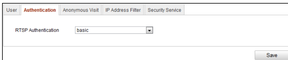
Figure 9-4 RTSP Authentication
