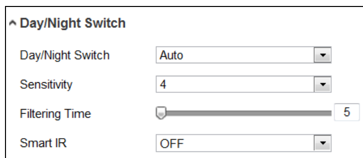
Figure 5-29 Day/Night Switch
