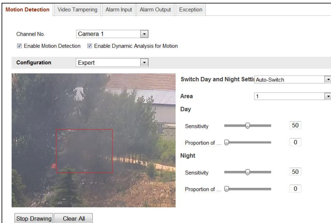
Figure 5-45 Day/Night Auto-Switch
