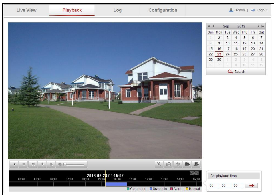
Figure 7-1 Playback Interface
