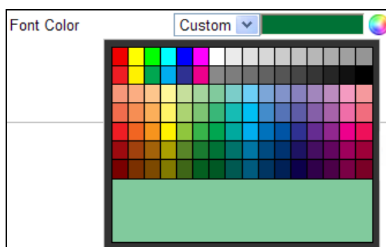
Figure 5-33 Font Color-Custom
