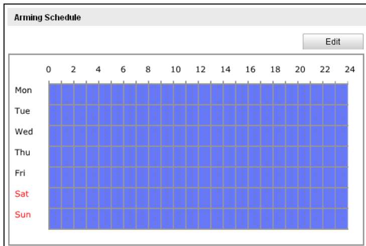
Figure 5-40 Arming Time
