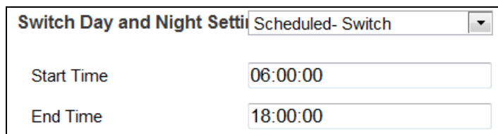
Figure 5-46 Day/Night Scheduled-Switch
