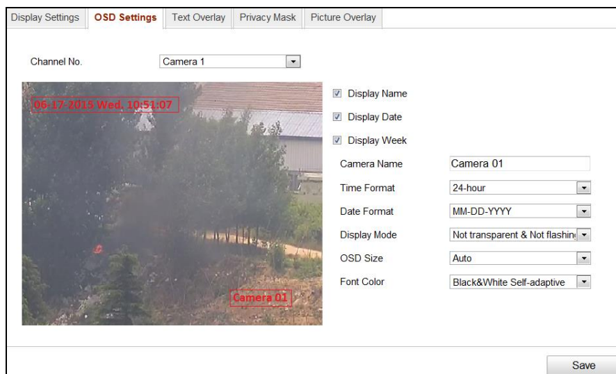
Figure 5-32 OSD Settings
