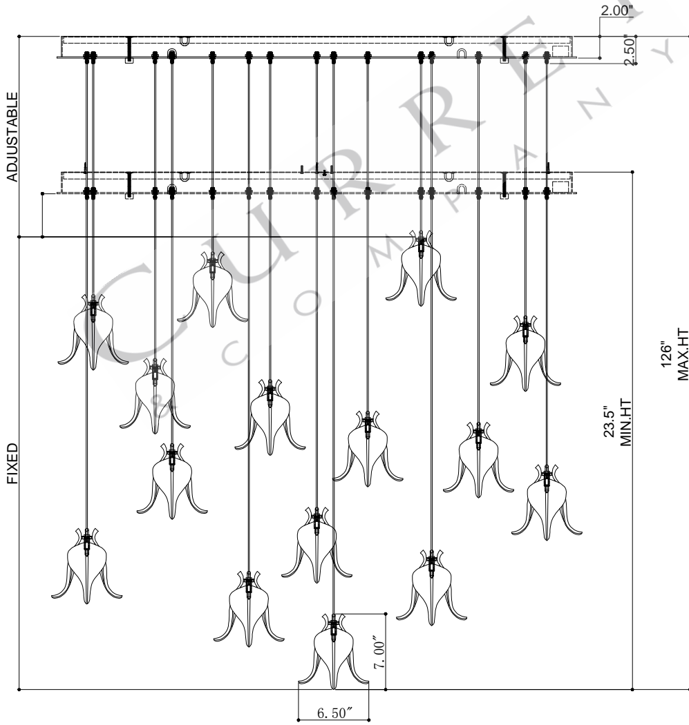
FRONT VIEW
