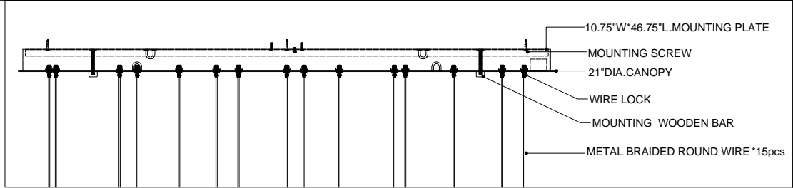
CANOPY DETAIL
