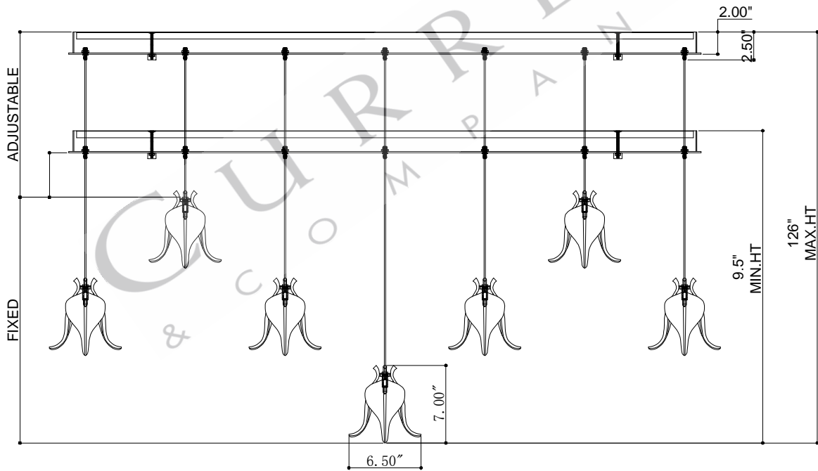
FRONT VIEW
