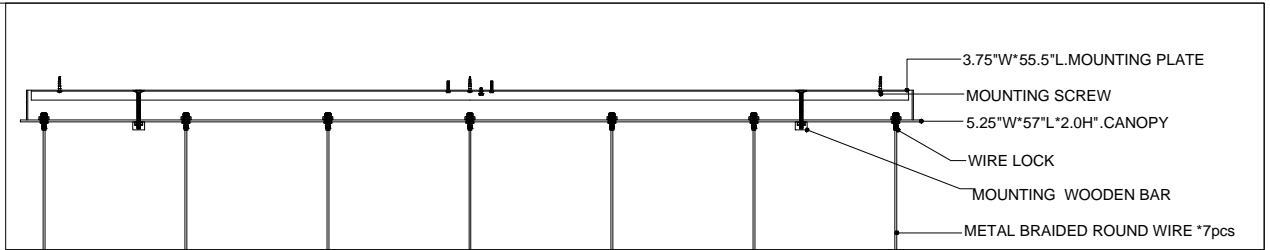
CANOPY DETAIL
