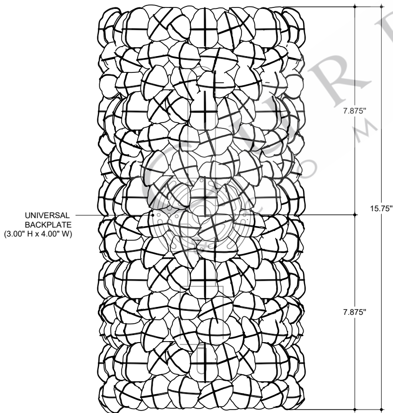
FRONT VIEW
