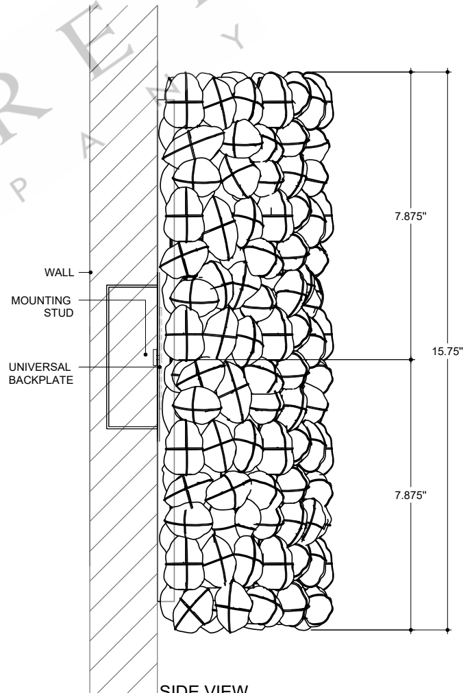
SIDE VIEW
