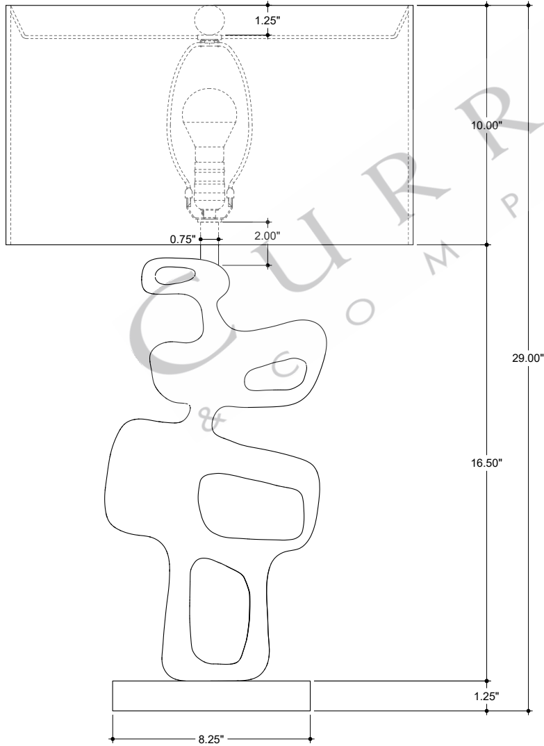
FRONT VIEW
