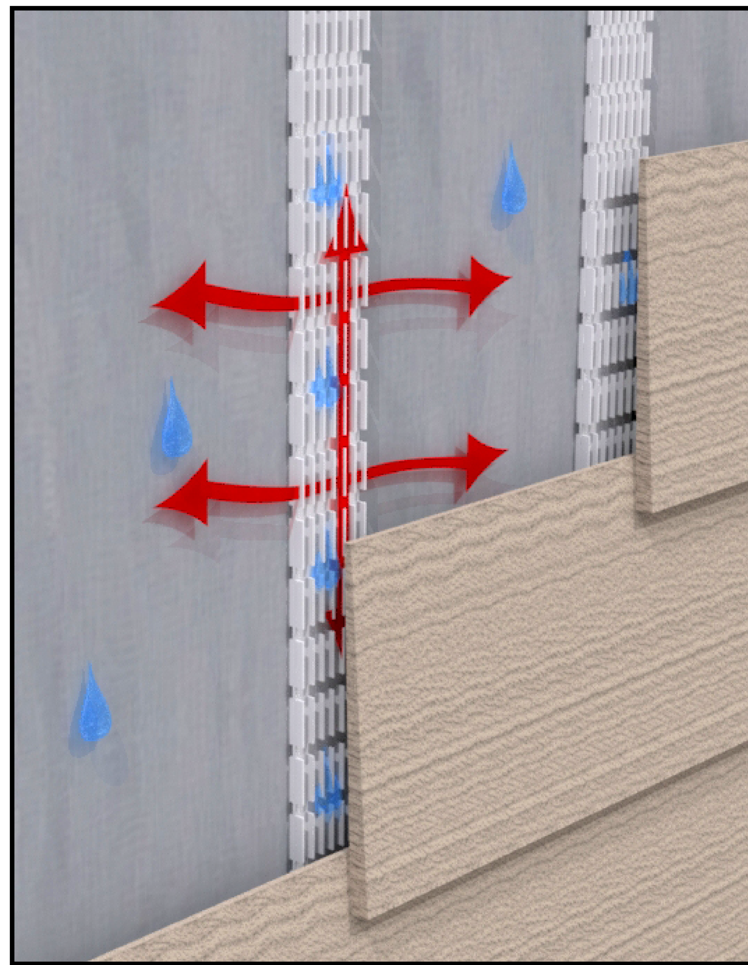
WATAIRVENT® VENTILATED FURRING STRIPS @16 IN. O.C.
