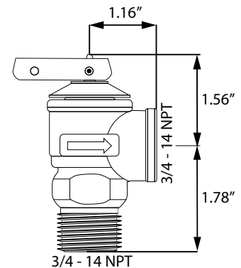
Pressure Relief Valve
