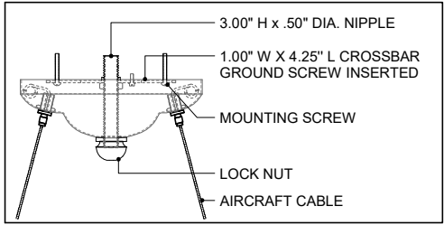
CANOPY DETAIL
