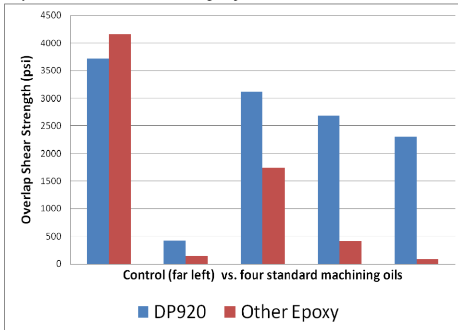
Figure 3. 3M™ Scotch-Weld™ Epoxy Adhesive DP920 vs. another toughened Scotch-Weld™ epoxy on oily cold rolled Steel.
