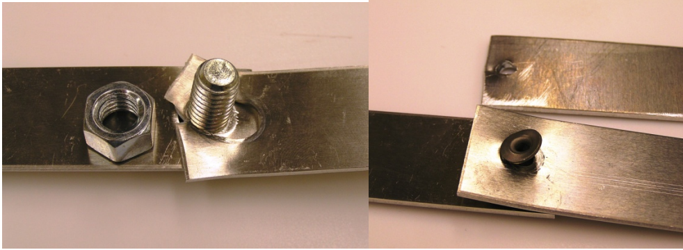
Figure 6. Failure of T6061 aluminum (0.063” thick) and rivets upon tensile force application vs. adhesively-bonded aluminum.
