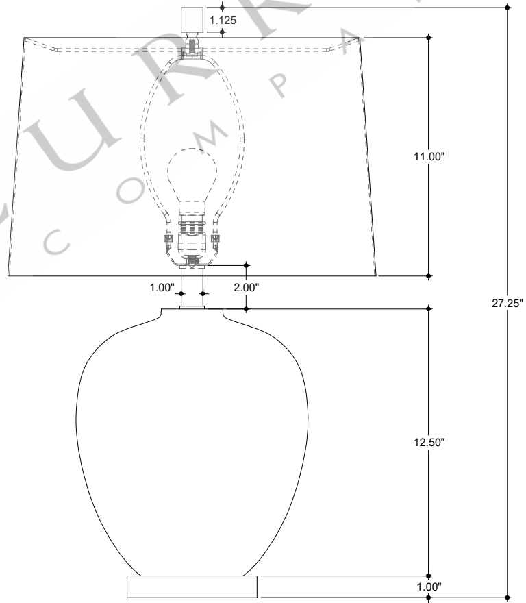
FRONT VIEW
