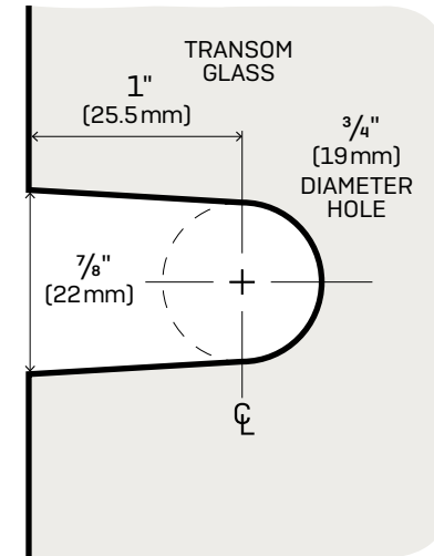
TEMPLATE OPTION FOR STANDARD FLAT POLISHED SQUARE CUT GLASS
