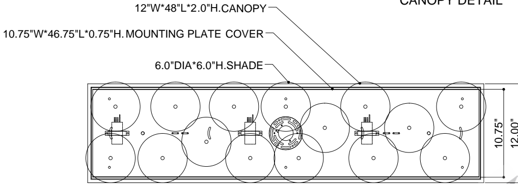
CANOPY DETAIL
