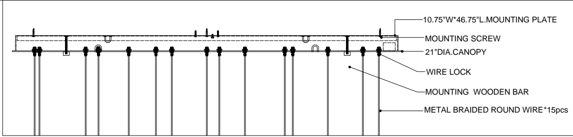
CANOPY DETAIL
