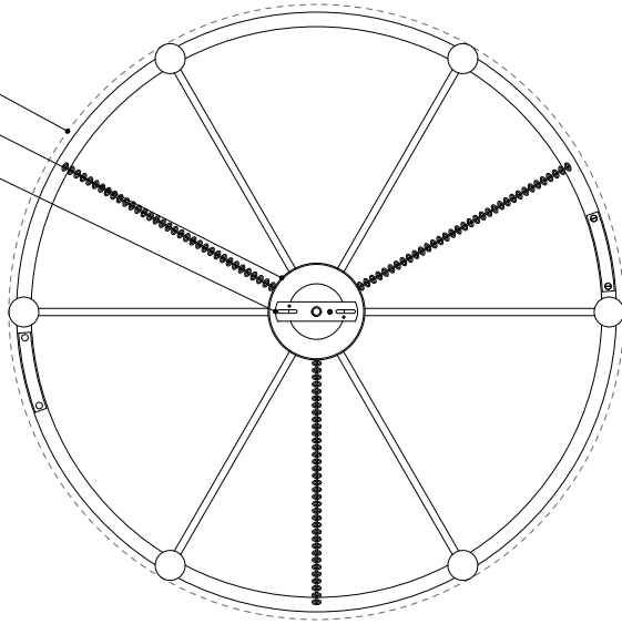
CANOPY DETAIL
