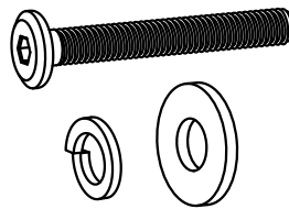
ALLEN KEY BOLT: M8 X 50mm - QTY 8 LOCK WASHER: Ø12 / Ø8 X 1.5mm - QTY 8 WASHER: Ø19 / Ø8 X 1mm - QTY 8
