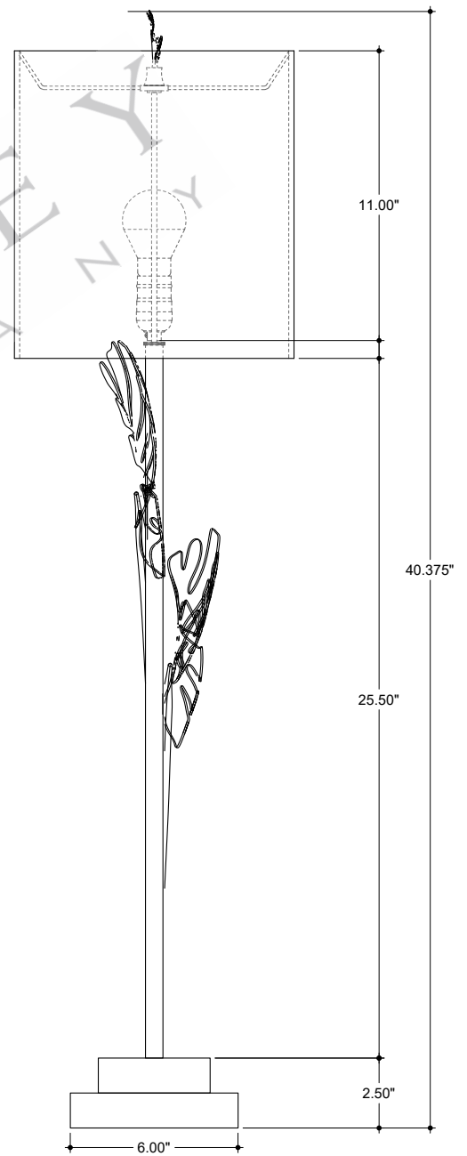
SIDE VIEW
