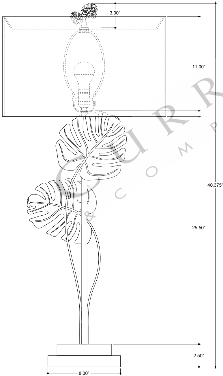
FRONT VIEW
