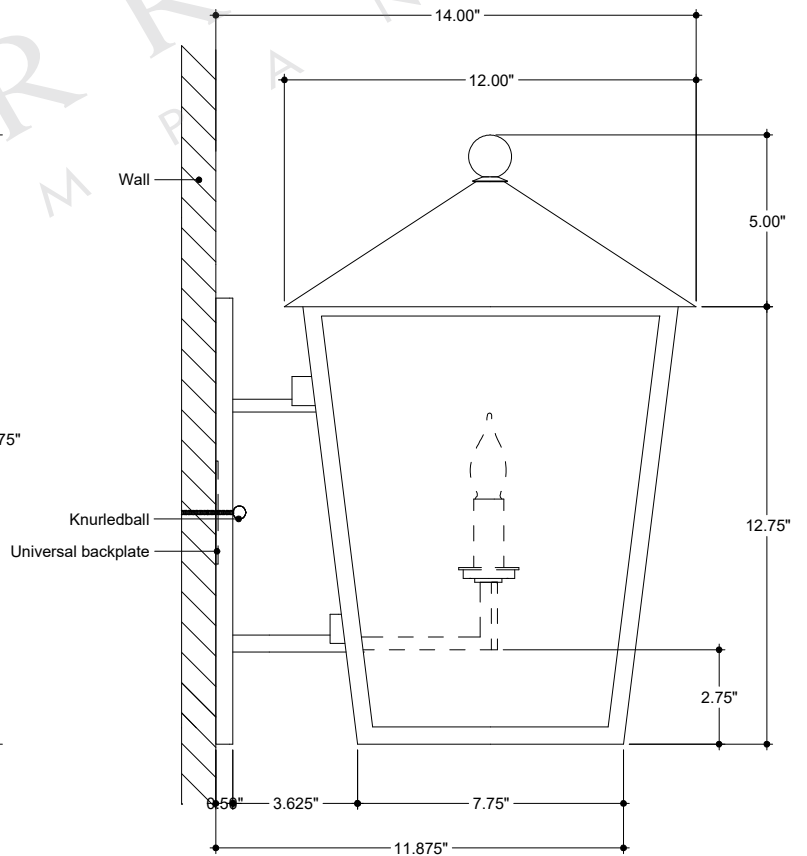
SIDE VIEW
