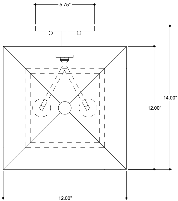
TOP VIEW
