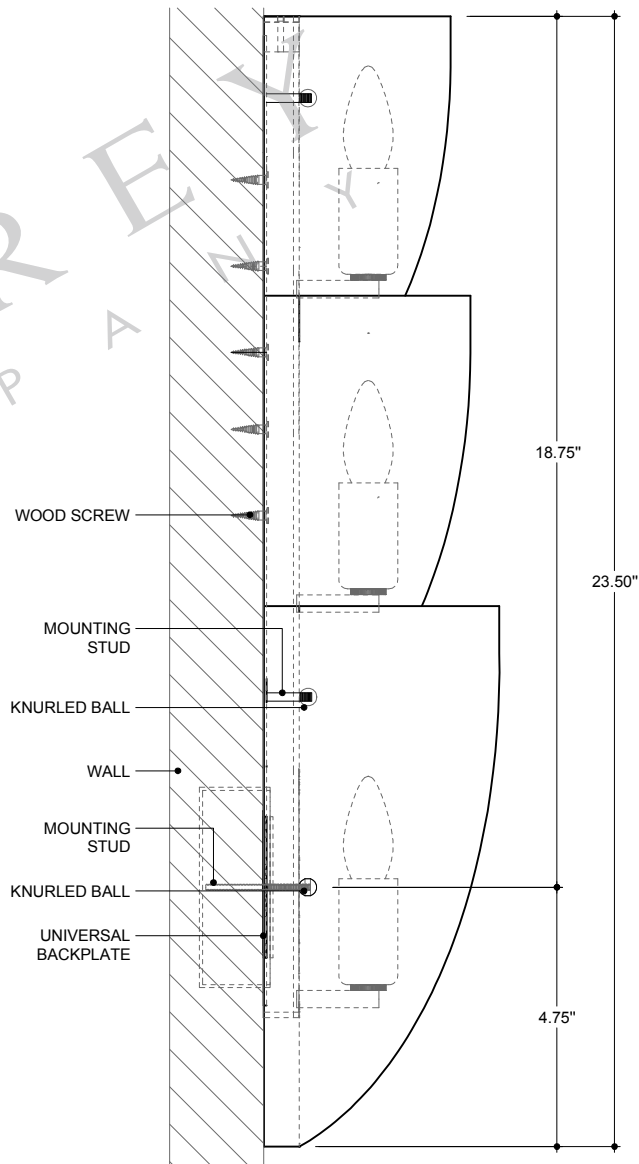
SIDE VIEW
