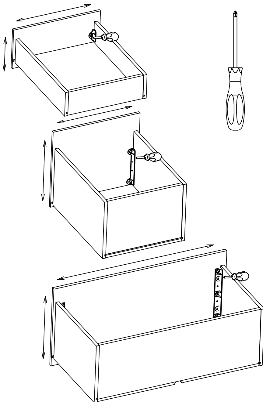
DRAWER FRONT VIEW
