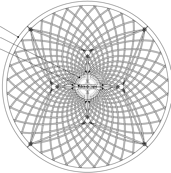
CANOPY DETAIL
