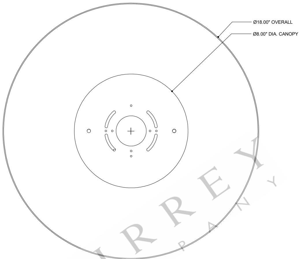
TOP VIEW
