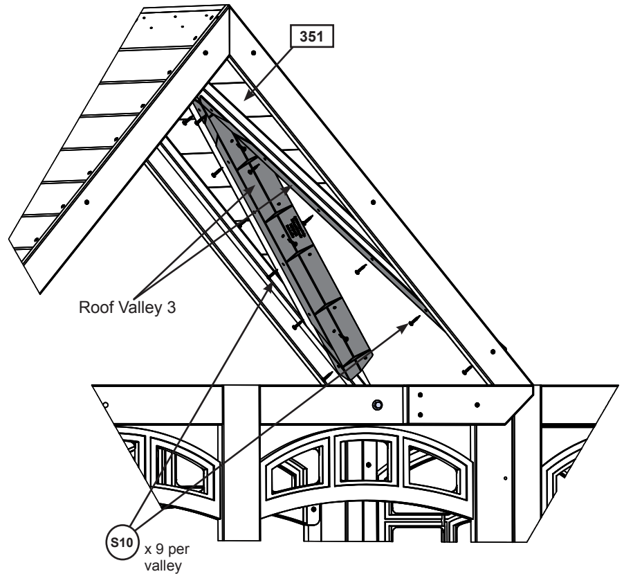
Fig. 37.4 Inside View
