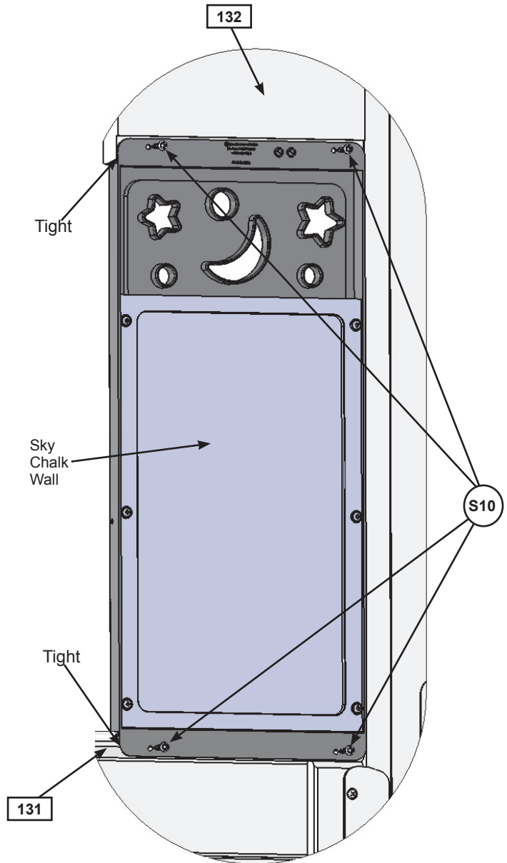
Fig. 13.7 Inside View
