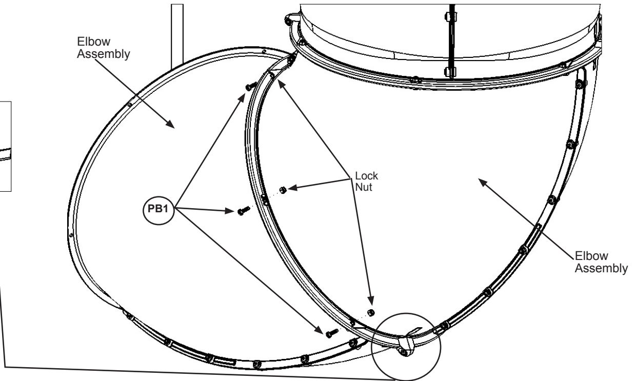
Fig. 27.2 Top Slide Bolt Holes
