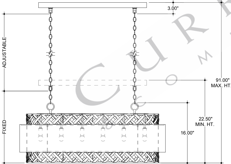
FRONT VIEW
