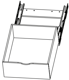
ROXXWB Rollout-Drawer
