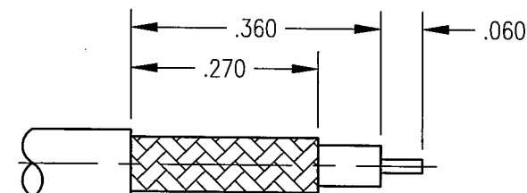
CABLE TRIMMING DIMENSIONS
