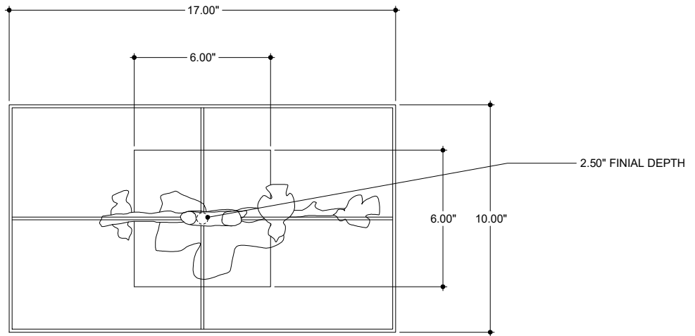
TOP VIEW
