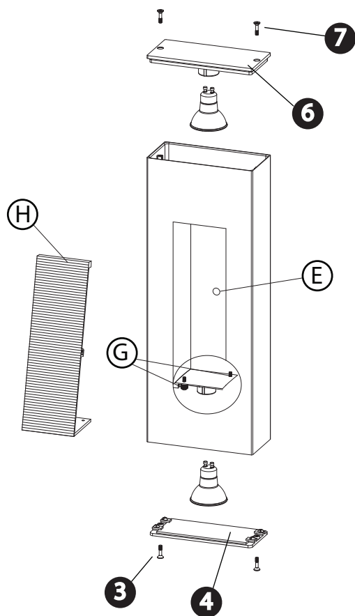
Drawing 2- Parts
