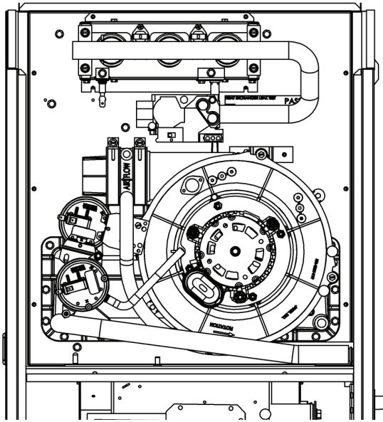
LEFT VENT - RIGHT DRAIN INSTALLATION
