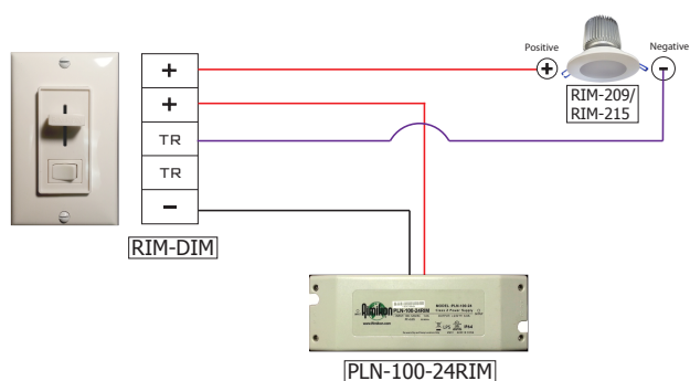
SINGLE DIMMER SWITCH WIRING
