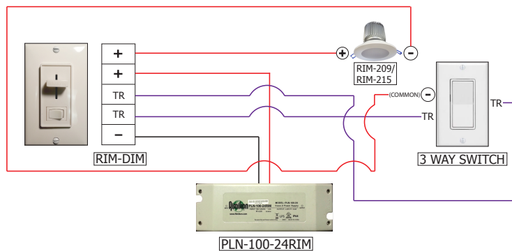
THREE WAY SWITCH AND DIMMER WIRING
